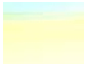
H0089 spectrum
